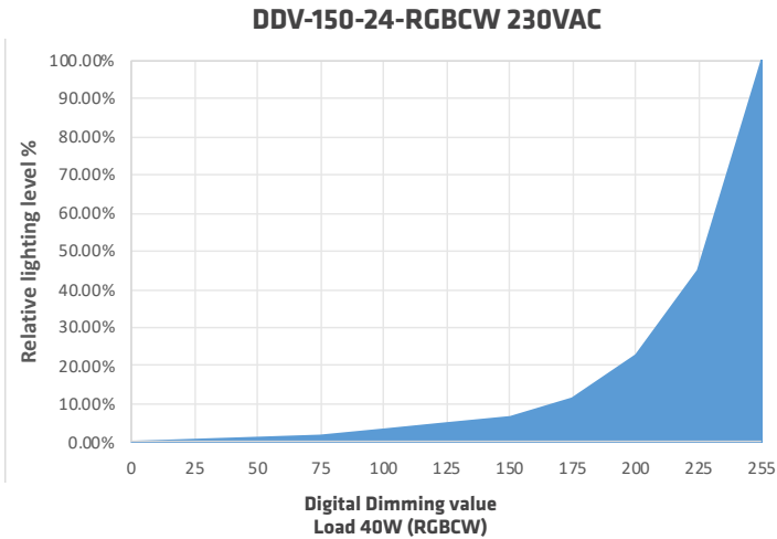
Illumination percentage test. Mode: DDV-150 230Vac Load: 40W(RGBCW)
