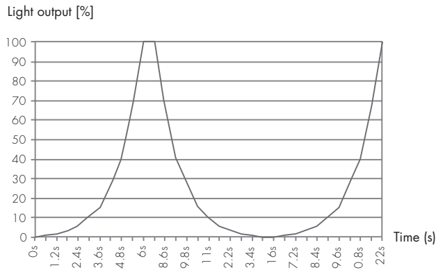
Switch-Dim Dimming Curve
