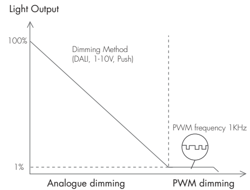
Dimming Profile
