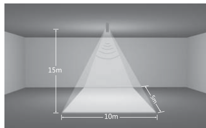
10m x 5m coverage @ 15m height (walk & stop) 6m x 4m coverage @ 15m height (continuous walking)
