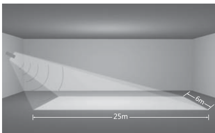
25m x 6m coverage @ 8m height
